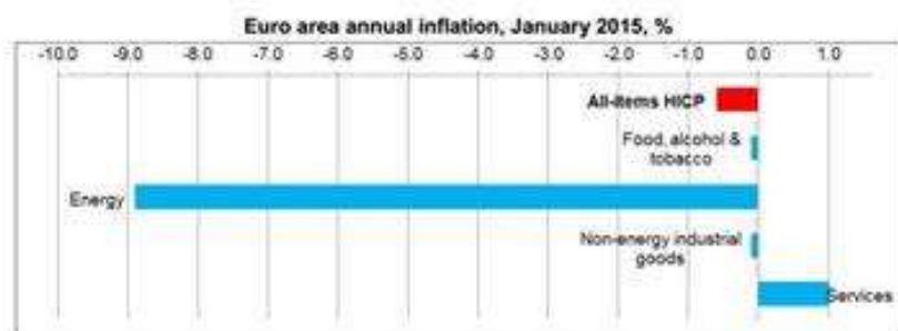
Euro area annual inflation and its components, %
